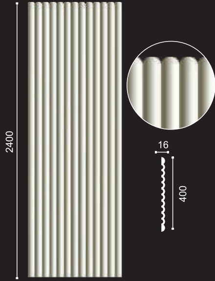
▲ PU-PNL-10 16x400x2400 mm
