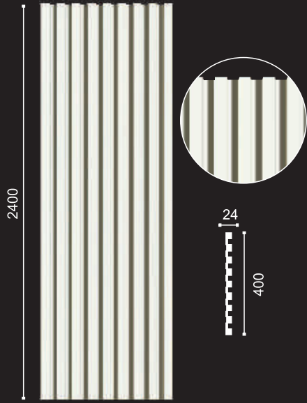
▲ PU-PNL-08 24x400x2400 mm
