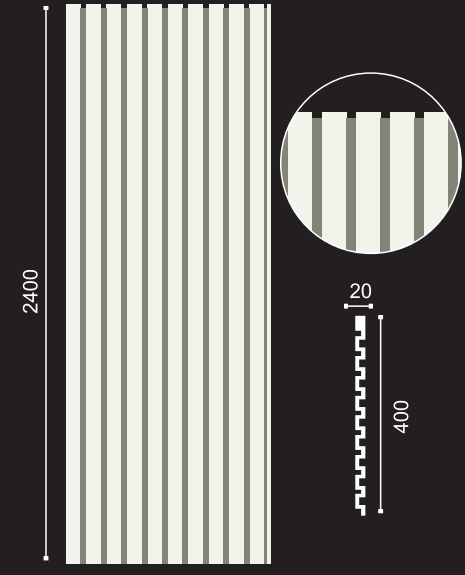
▲ PU-PNL-17 20x400x2400 mm
