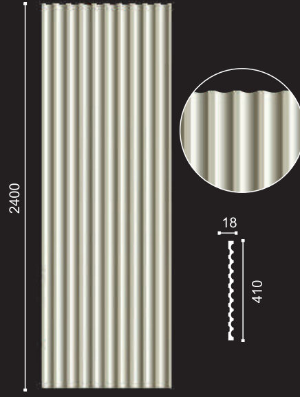
▲ PU-PNL-09 18x410x2400 mm
