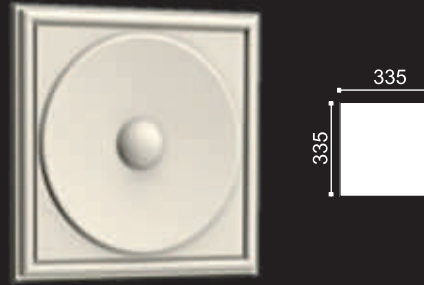
▲ PU-DP-330 335x335 mm
